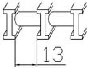
AluRoll/Fix250/13
